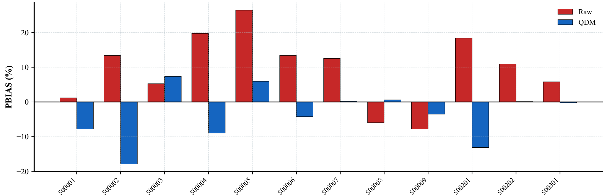
Spatial variation of PBIAS across stations — independent validation
